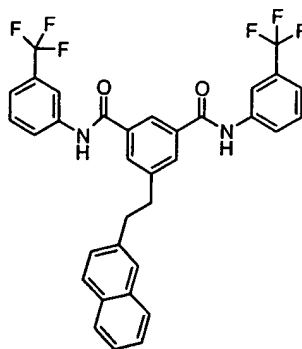
Compound # 24
